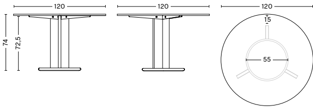
CHISEL 29 TABLE | COLUMN Diameter 120 cm Height 74 cm Weight 50 kg
