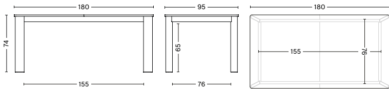
CHISEL 630 TABLE Length 180/280 cm Width 95 cm Height 74 cm Weight 87 kg
